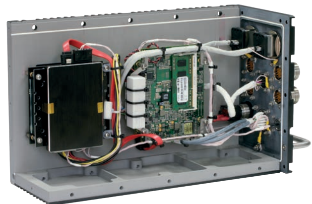
M-Max ATR-chassis
